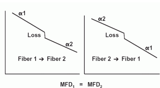
Fig. 11 Two bidirectional OTDR traces showing a splice between fibers with unequal fiber attenuations ( \alpha_1 > \alpha_2 ) and a true splice loss. Because of the assumed equal mode fields both traces show the same true loss.
