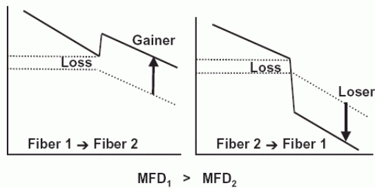
Fig. 12 The same two bidirectional OTDR traces, now assuming difference in mode ( MFD_1 > MFD_2 ), causing an equal “Loser” and “Gainer”, which - due to the presence of true loss - are unequally shown by the OTDR.
