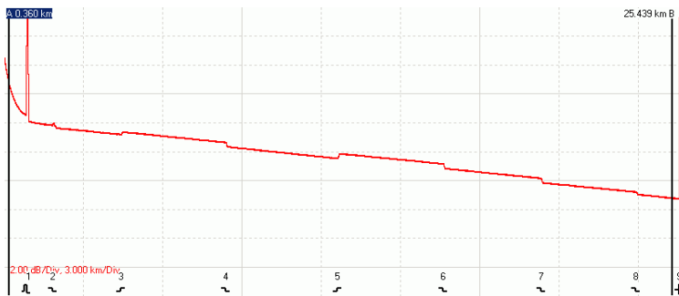
Fig. 9 Example of an OTDR for field use. Typical OTDR trace with splices, including "gainers"
