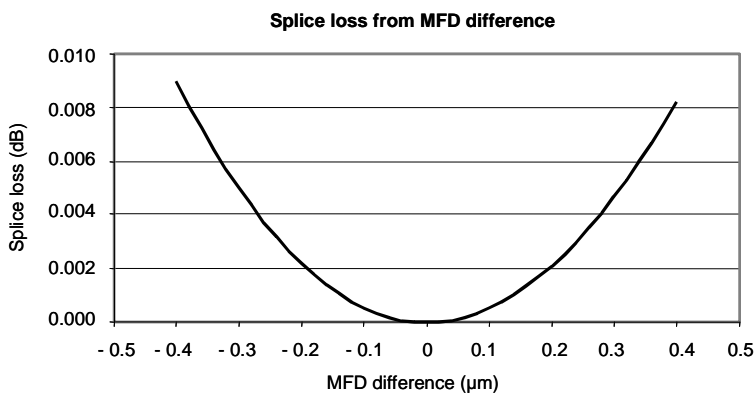
Fig. 7 True splice loss due to MFD difference
