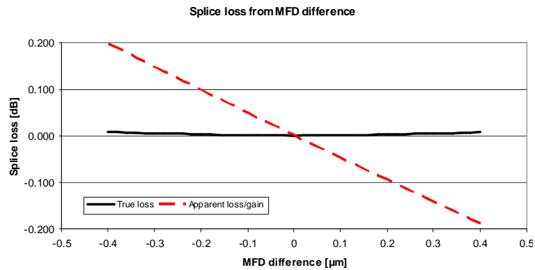
Fig. 10 Error in unidirectional OTDR measurements (apparent gain or loss) in comparison to true splice loss due to MFD difference
